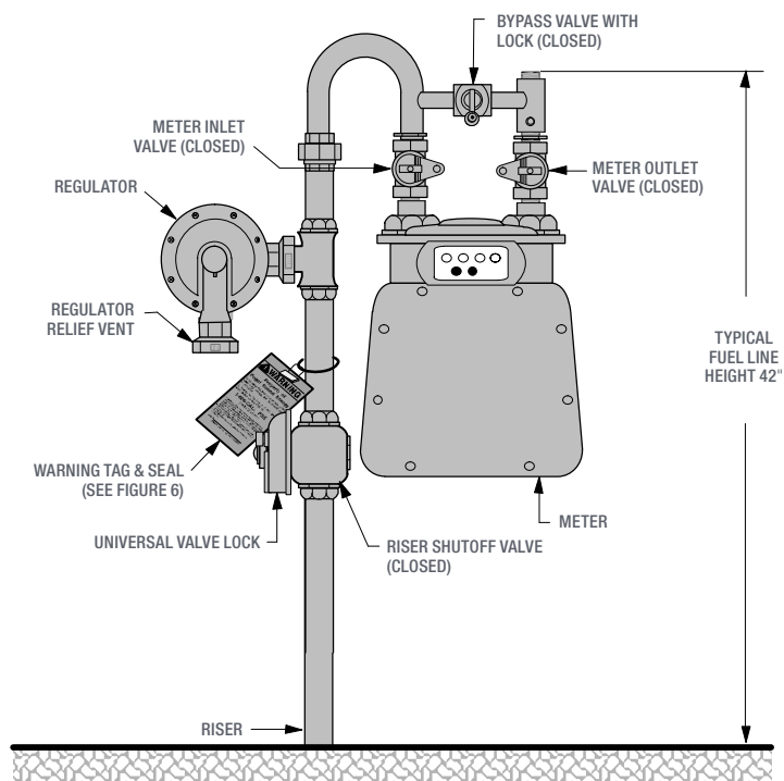
Figure 8 Typical 425 through 1000 gas meter set assembly
