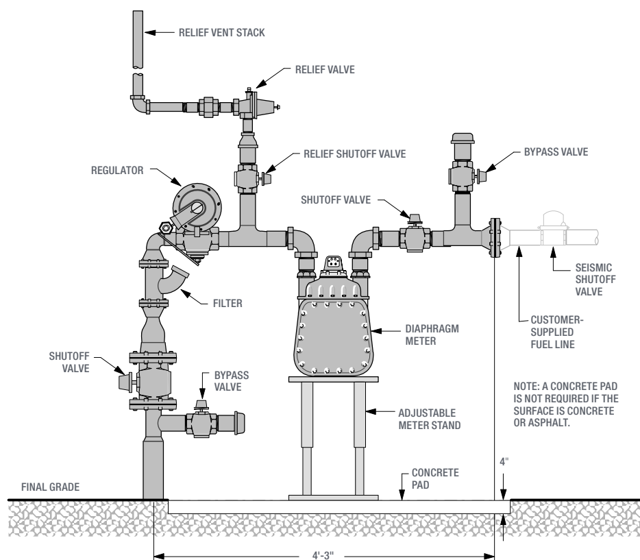
Figure 3 Typical commercial/industrial diaphragm-type gas meter set assemblies
