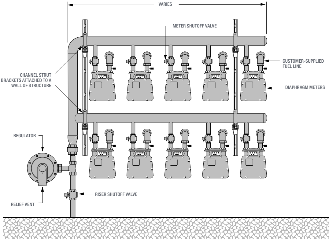
Figure 5 Components of a typical 250 manifold meter set assembly for a commercial structure with multiple tenants or multifamily
