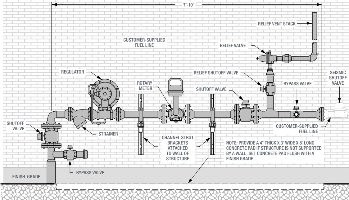
Figure 4 Typical commercial/industrial rotary-type gas meter set assemblies
