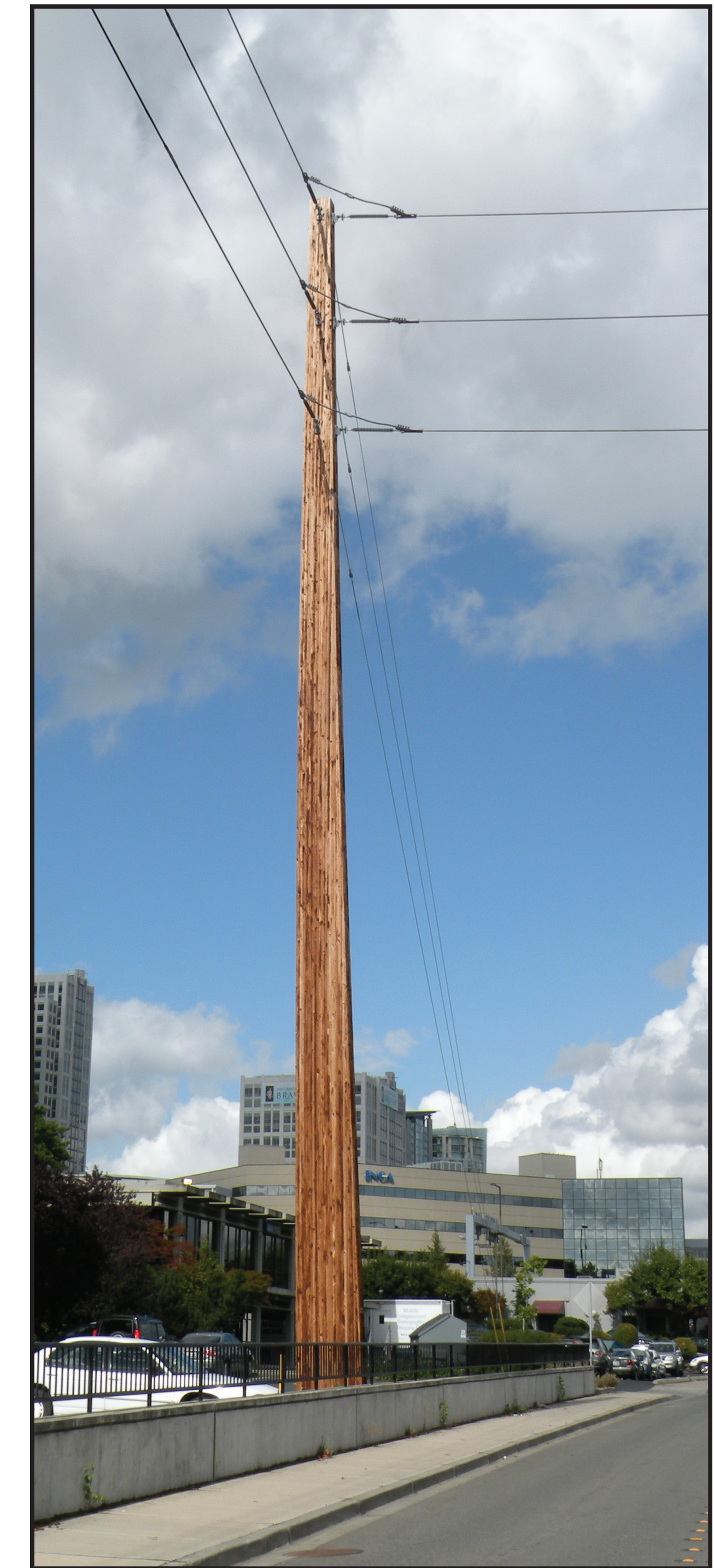
Single-circuit 115 kV glu lam pole
